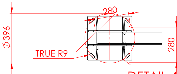
DETAIL A SCALE 1 : 15
