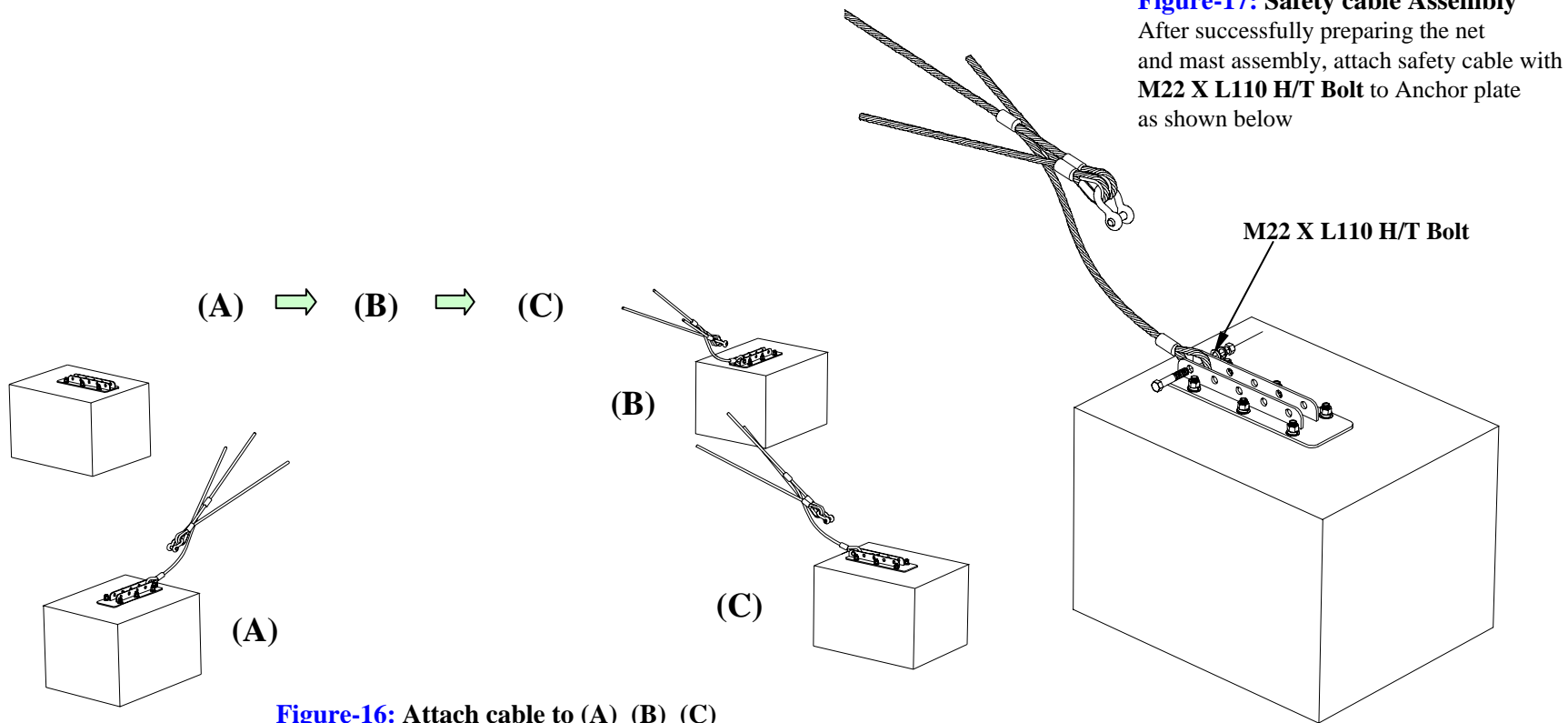
Figure-16: Attach cable to (A) (B) (C)
