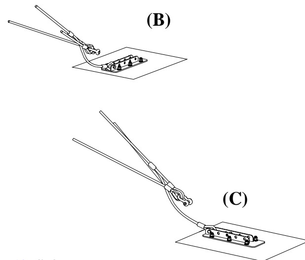
Figure-19: Safety cables attached
