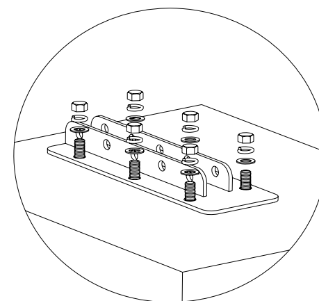
(b) Post plate
