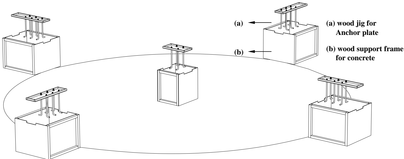
Figure-6: Wood support frame
