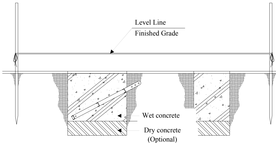
Figure-4: Foundation section view
