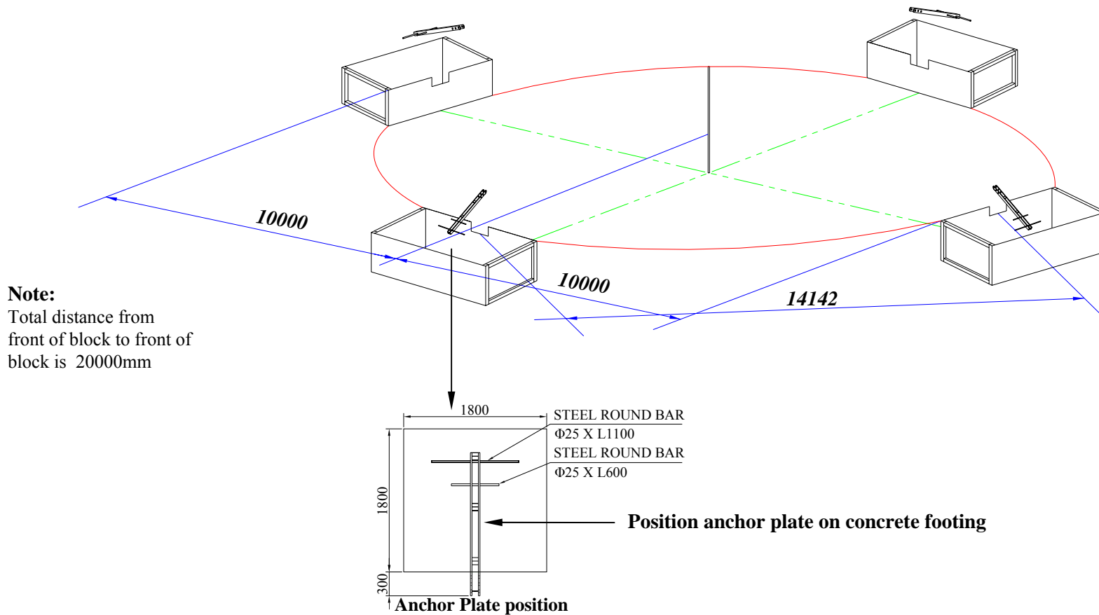
Figure -5: Footing and anchor plate layout
