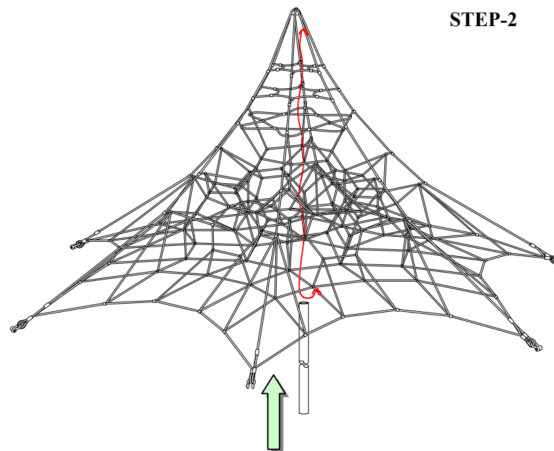
Figure-12: Insert Post following Nylon string
