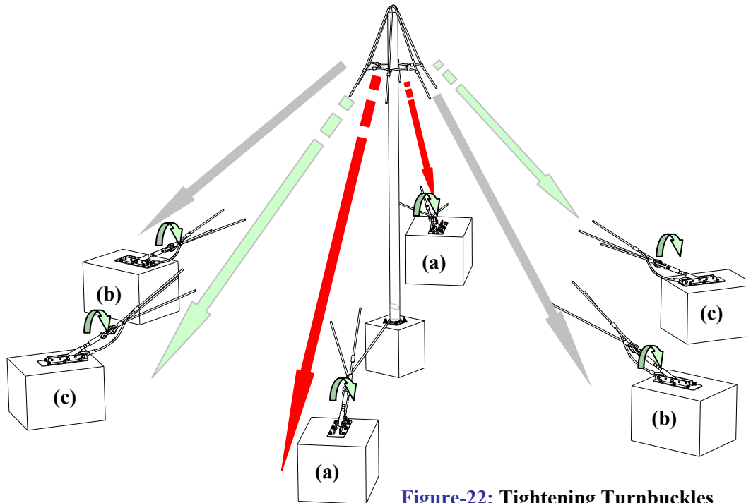
Figure-22: Tightening Turnbuckles
